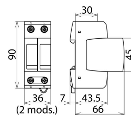
Dimension drawing DG M TT 2P 275 NL
