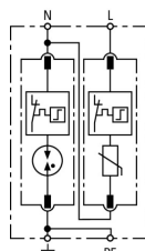
Basic circuit diagram DG M TT 2P 275 NL
