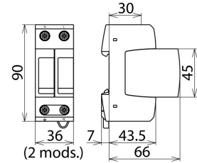
Dimension drawing DG M TT 2P 275 NL
